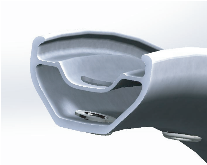
Tech XC Rim Profile
