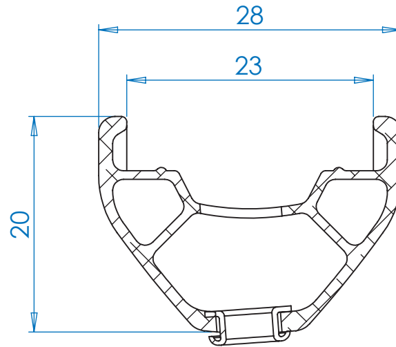
Tech Enduro Rim Profile
